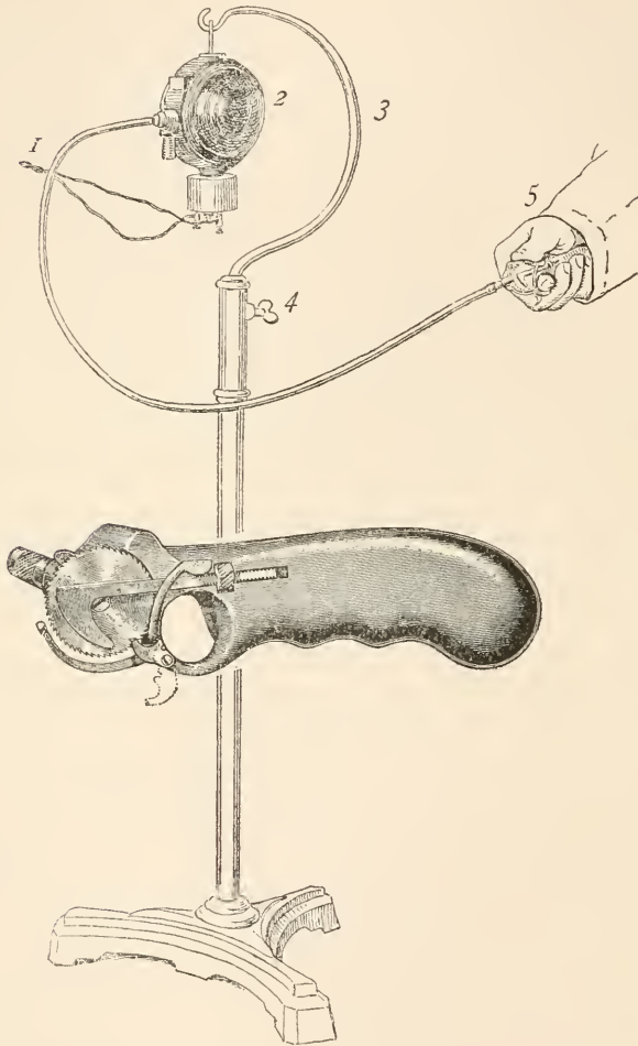
FIG. 27.—Masland's electric saw and stand. 1, electric wiring; 2, electric motor; 3, curved portion of support; 4, means for elevating motor; 5, saw in use.
